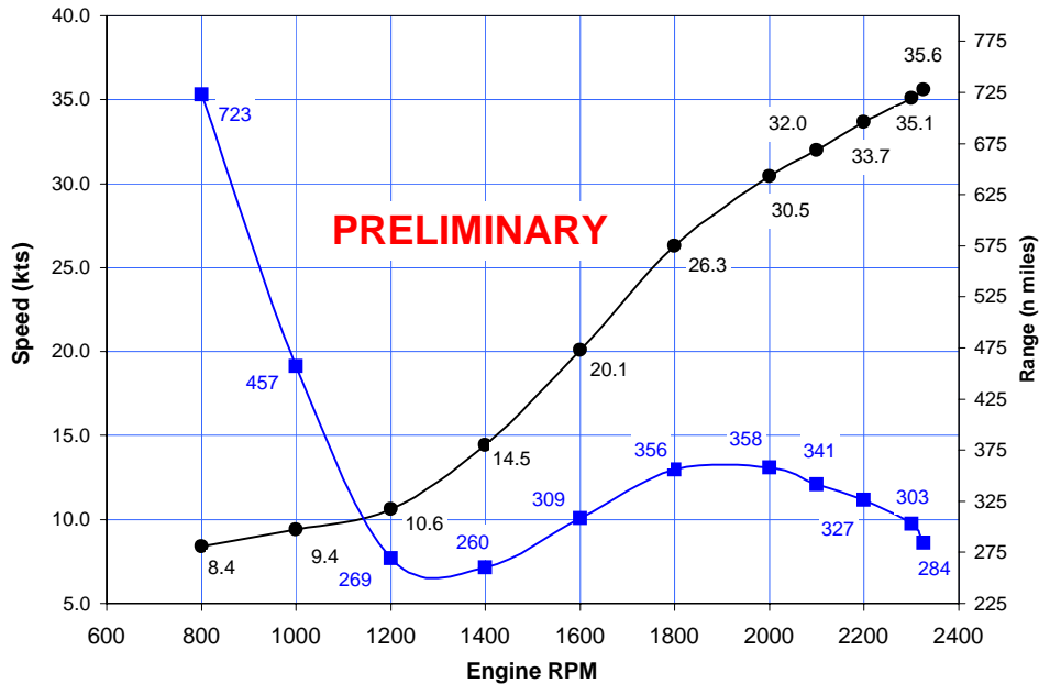
Cabo 40 Flybridge 01 - CAT C12 522kW / 700HP SAE / 710HP M ZF325A 1.485:1 Michigan HX400, 26x32 4B, Nibral, 0.85 DAR, #3 Cup
