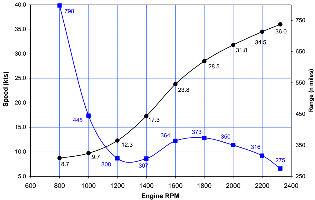
Cabo 40 Express 014 - CAT C12 522kW / 700HP SAE / 710HP M ZF325A 1.485:1 Michigan HX400, 26x32.5 4B, Nibral, 0.85 DAR, #3 Cup
